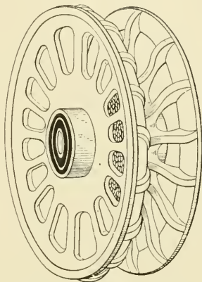
Fig. 107. Special Form of Trolley Wheel for Cutting Sleet
